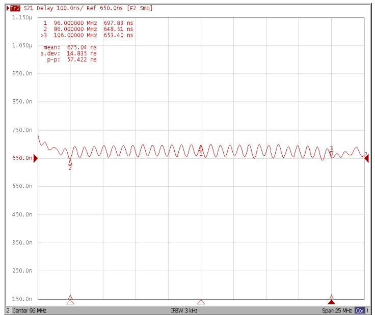
Group Delay Variation (86.0~106MHz)
